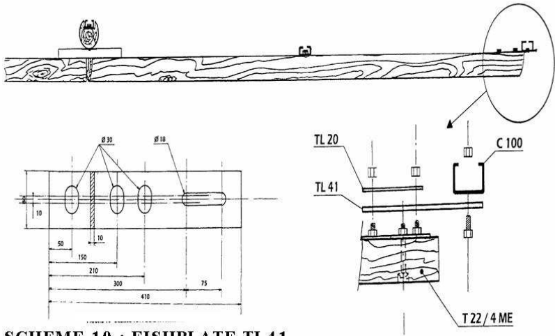
SCHEME 10 : FISHPLATE TL41 OF THE ANCHOR SYSTEM
