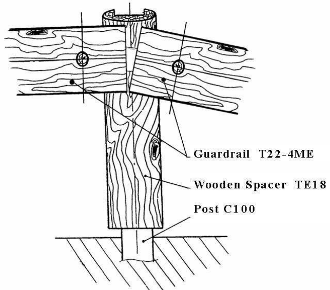
SCHEME 8 : CONNECTION OF THE ANCHOR SYSTEM
